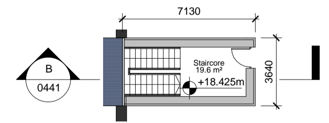
5 Fourth Floor Plan 1 : 200
