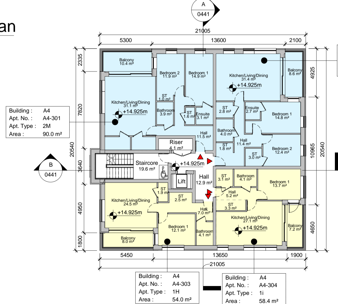
4 Third Floor Plan 1 : 200
